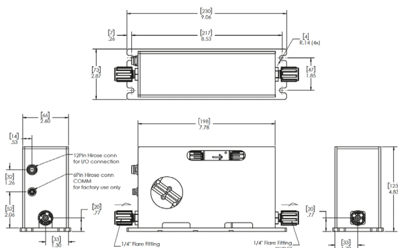
Dimensions for 1/4" Flare end connections
