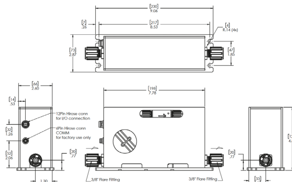
Dimensions for 3/8" Flare end connections
